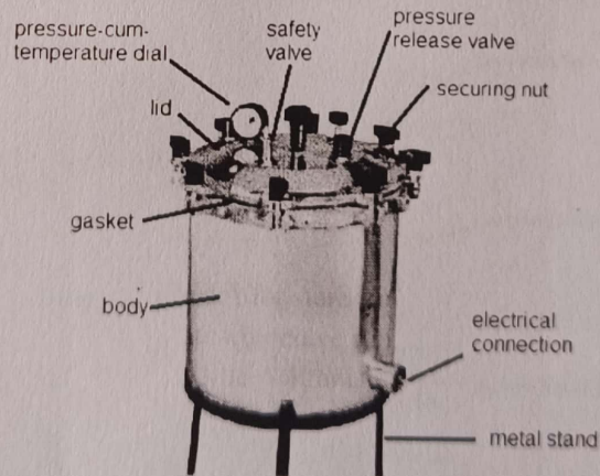
Fig 1 Portable autoclave
