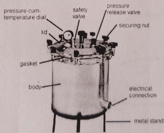
Fig 1 Portable autoclave
