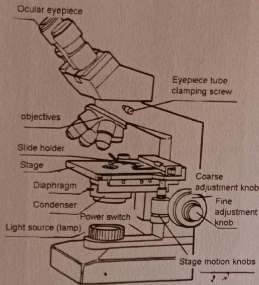
Fig. 13 Compound microscope
