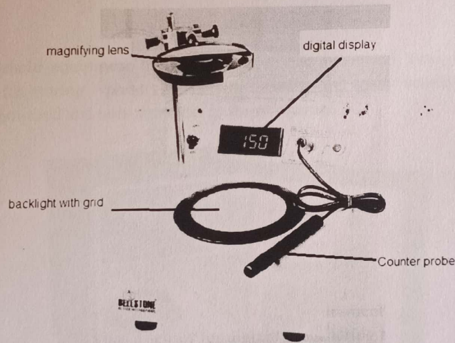
Fig. 12 Colony counter
