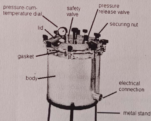
Fig 1 Portable autoclave
