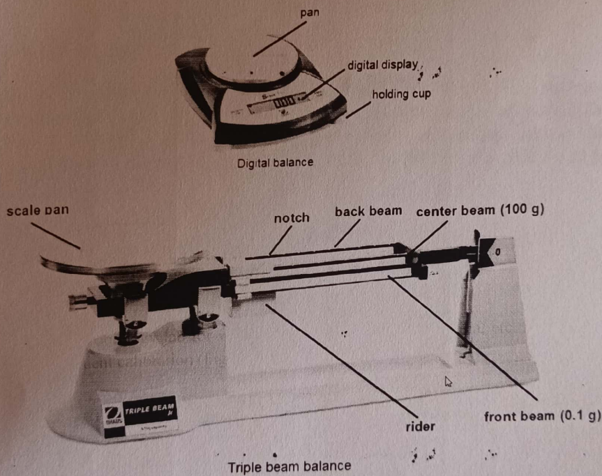
Fig. 18 Different types of balances
