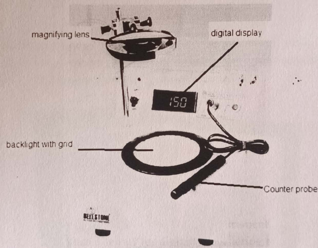
Fig. 12 Colony counter
