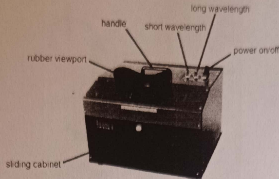
Fig. 9 UV viewing cabinet
