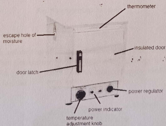
Fig. 3 Hot air oven
