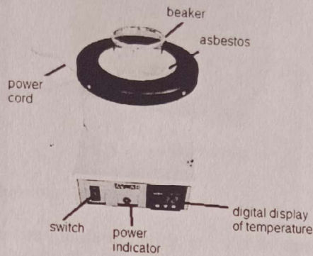
Fig. 7 Heating mantle
