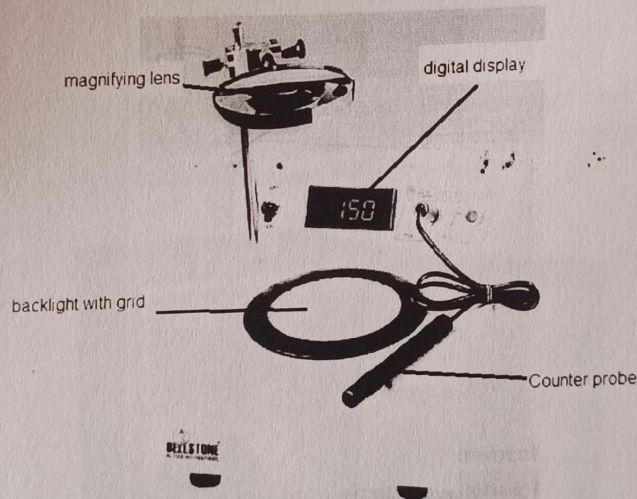
Fig. 12 Colony counter
