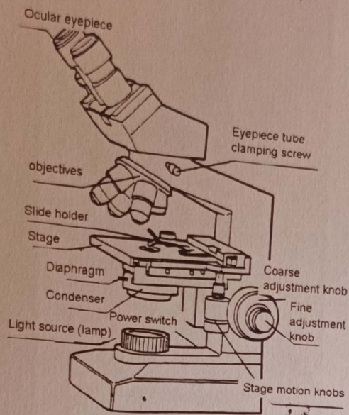
Fig. 13 Compound microscope
