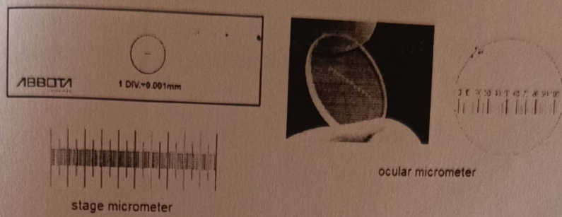
Fig. 17 Stage and ocular micrometer
