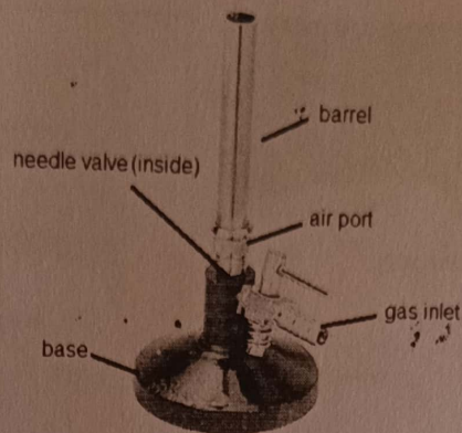
Fig 15 Bunsen burner
