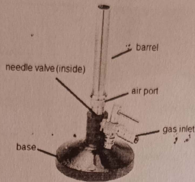
Fig 15 Bunsen burner
