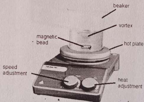
Fig. 8 Hot plate with magnetic stirrer
