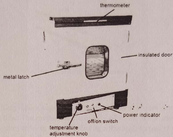
Fig. 2 Incubator
