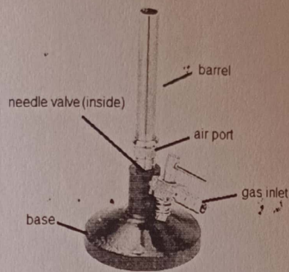
Fig 15 Bunsen burner
