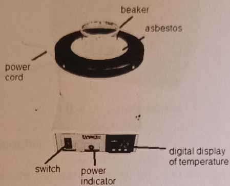
Fig. 7 Heating mantle
