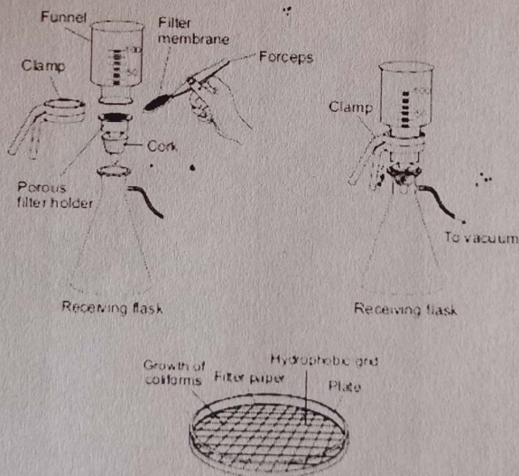
Fig. 20 Coliform membrane filter
