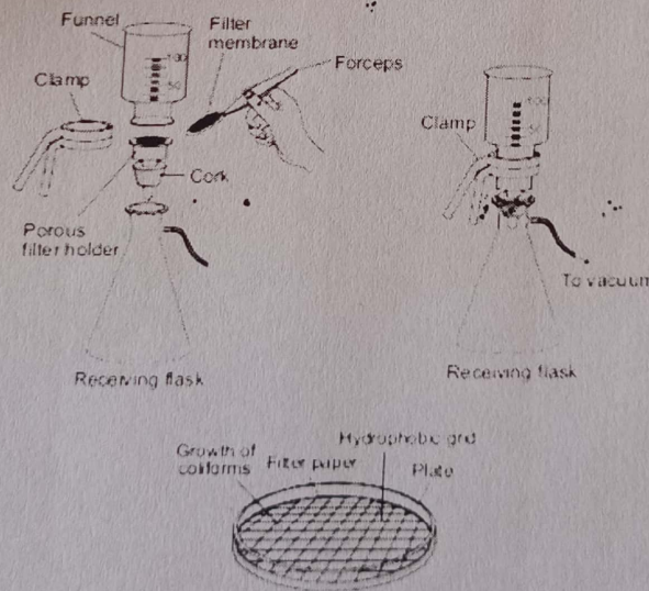
Fig. 20 Coliform membrane filter
