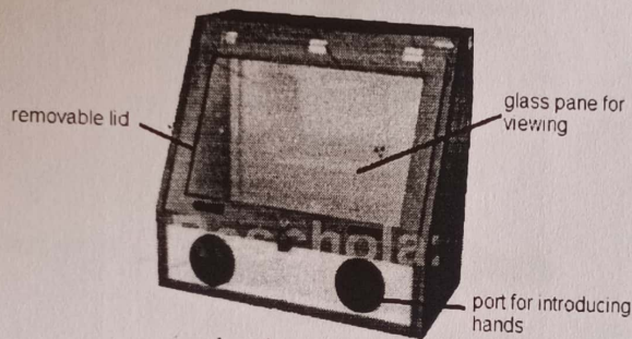
Fig. 10 Inoculation chamber
