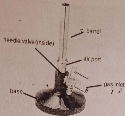
Fig 15 Bunsen burner
