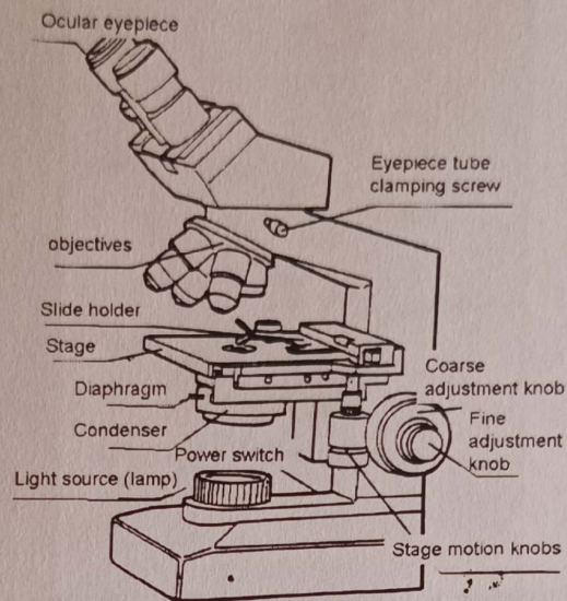
Fig. 13 Compound microscope
