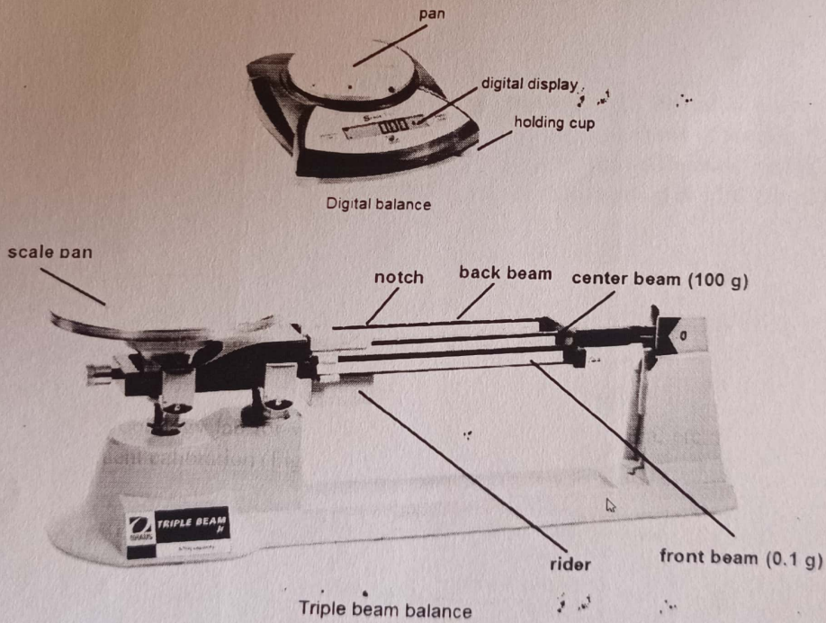
Fig. 18 Different types of balances
