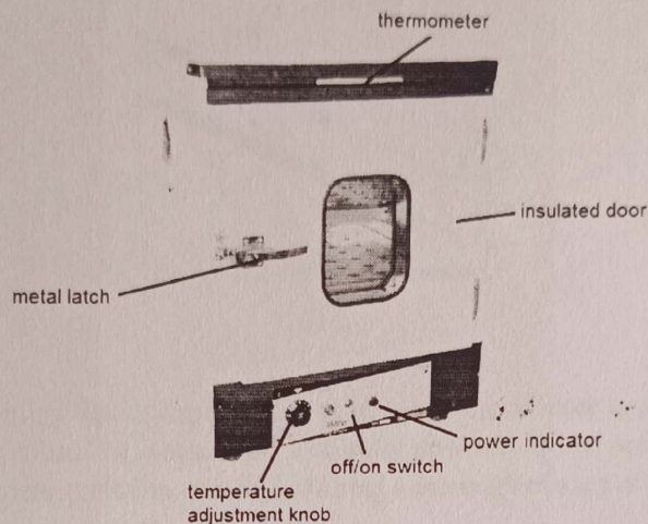
Fig. 2 Incubator
